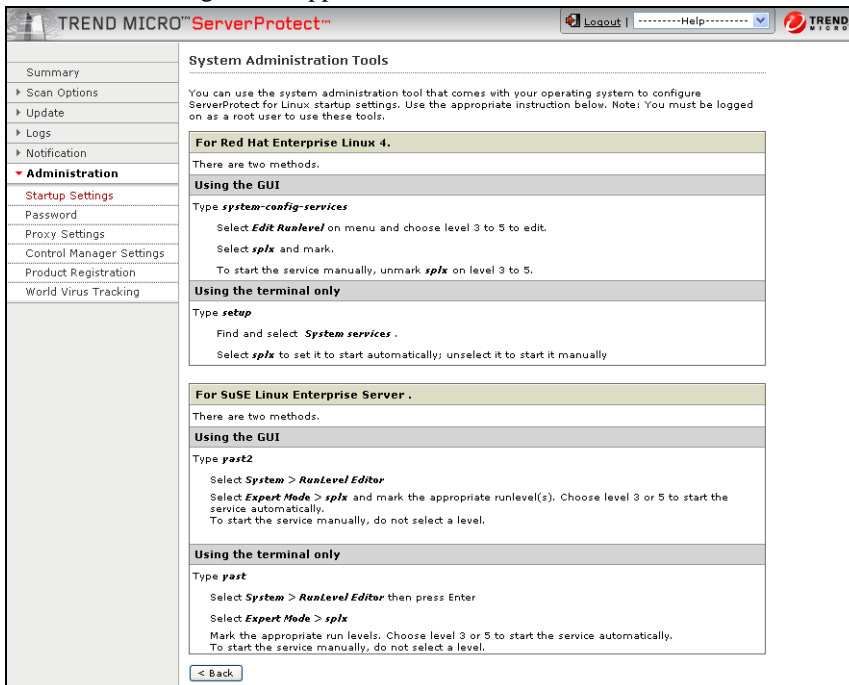
FIGURE 2-3. Administration: Startup Settings
