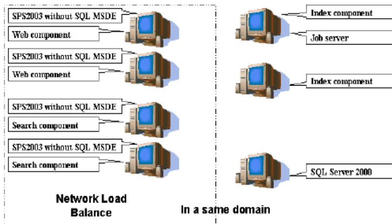
FIGURE 2-3. Large server farm configuration
