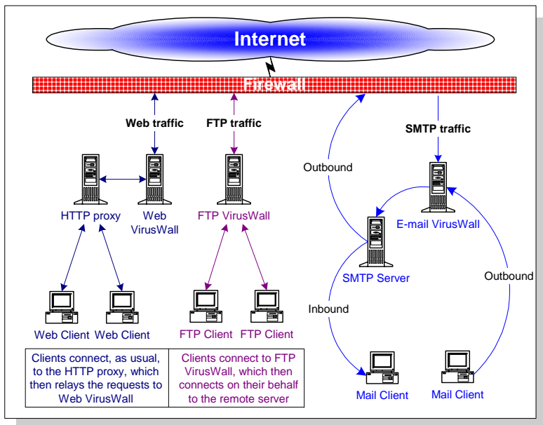
FIGURE 3-1. Sample installations of the Standard edition of Web, FTP, and Email VirusWall on a LAN.
