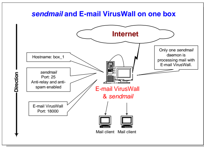
FIGURE 6-7. sendmail daemon and InterScan VirusWall running on the same machine.
