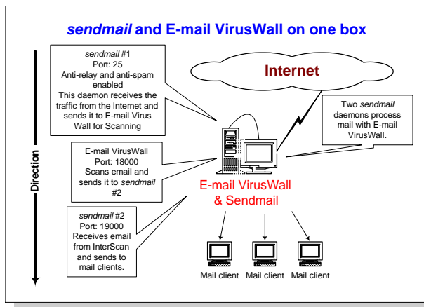
FIGURE 6-8. The illustration shows two sendmail daemons and InterScan VirusWall on the same Unix box.
