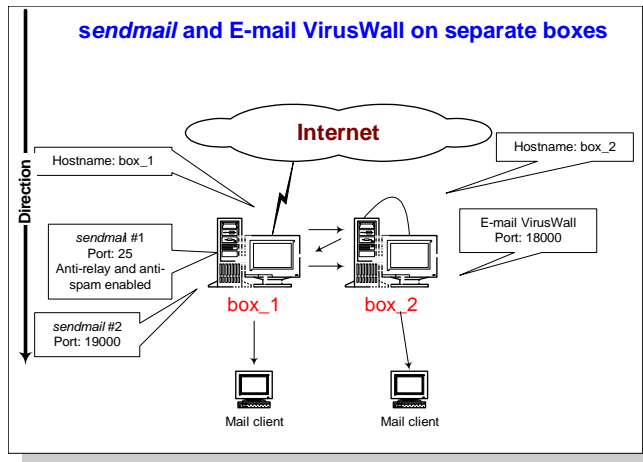
FIGURE 6-9. Two Unix boxes configured to handle SMTP traffic. The arrows show the flow of traffic between boxes.
