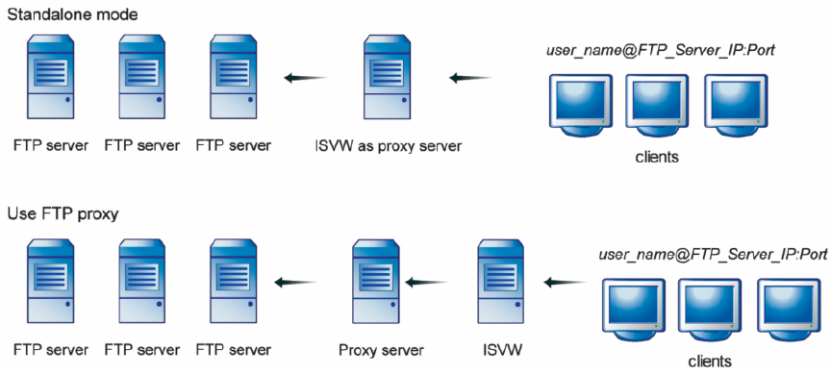
FIGURE 2-4. Installation Topology for FTP with Proxy Server
