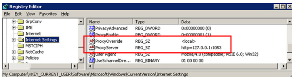
Figure 3. Registry entries some FAKEAV variants create to ensure that Internet browser requests are intercepted
