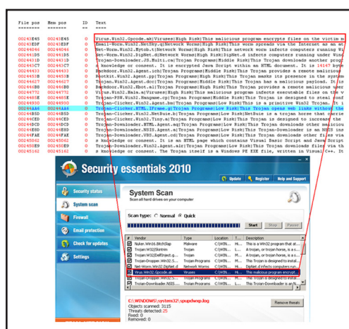
Figure 2. Fake infection hard-coded into the FAKEAV malware's body
